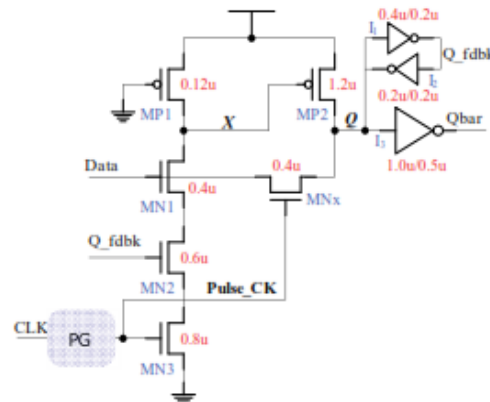
Fig (e) Modified circuit
