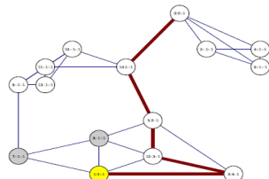
Example DFS
