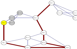
Example DFS
