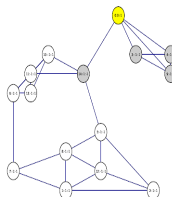
Example DFS
