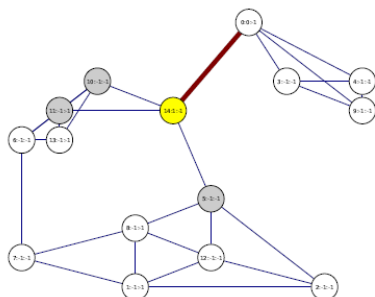
Example DFS
