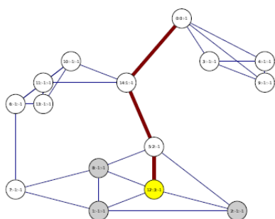
Example DFS
