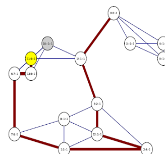
Example DFS
