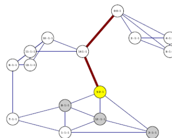
Example DFS
