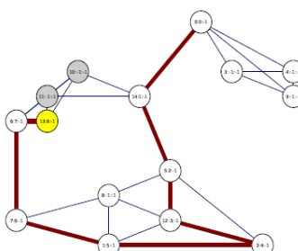
Example DFS
